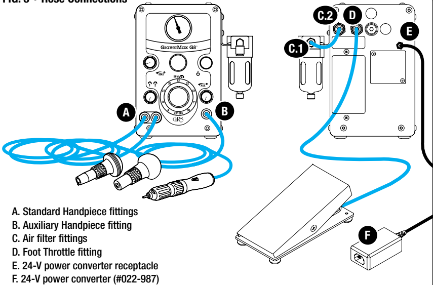
FIG. 3 • Hose Connections
